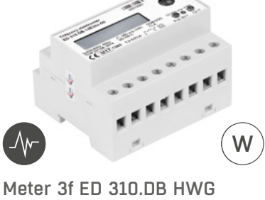
Meter 3f ED 310.DB HWG 3× 230 V/400 V, 63 A
