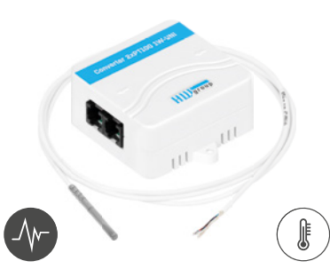
Temp-1W-UNI Pt100 Frost Temperature range: -190 to 150 °C, Converter 2xPt100 1W-UNI
